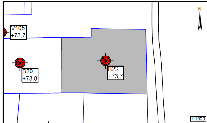
Figur 1 – Situationsplan 1:1000, Hvedebakken 22
