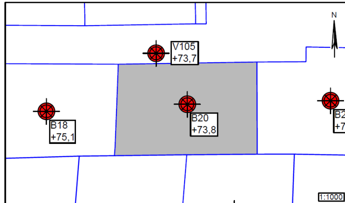
Figur 1 – Situationsplan 1:1000, Hvedebakken 20
