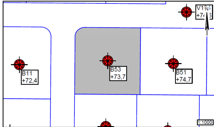
Figur 1 – Situationsplan 1:1000, Hvedebakken 53
