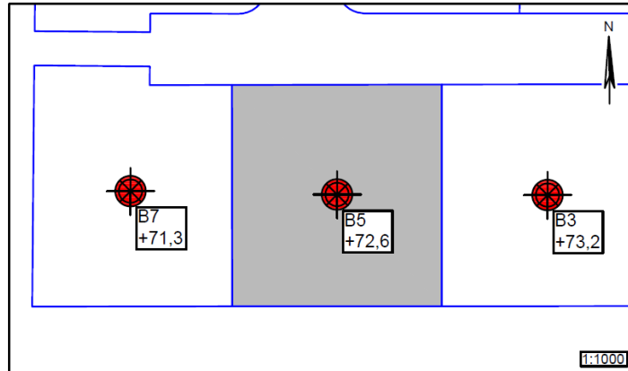
Figur 1 – Situationsplan 1:1000, Hvedebakken 5
