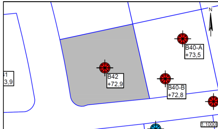
Figur 1 – Situationsplan 1:1000, Hvedebakken 42
