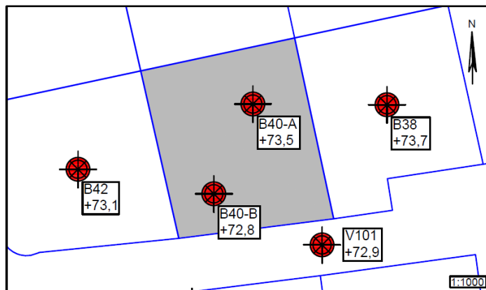
Figur 1 – Situationsplan 1:1000, Hvedebakken 40
