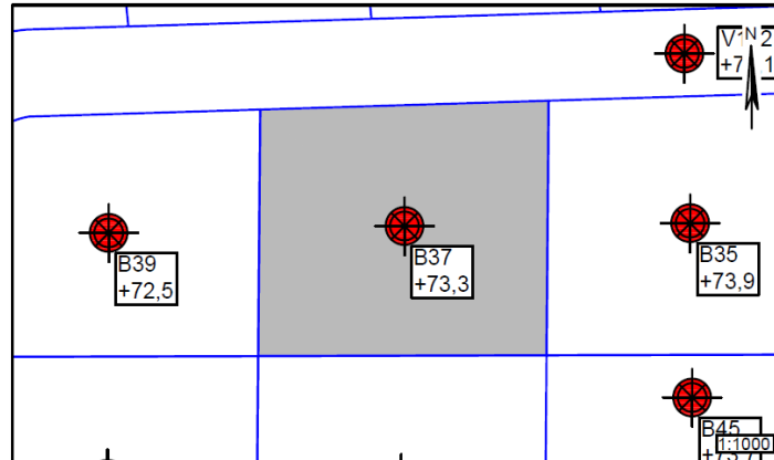
Figur 1 – Situationsplan 1:1000, Hvedebakken 37
