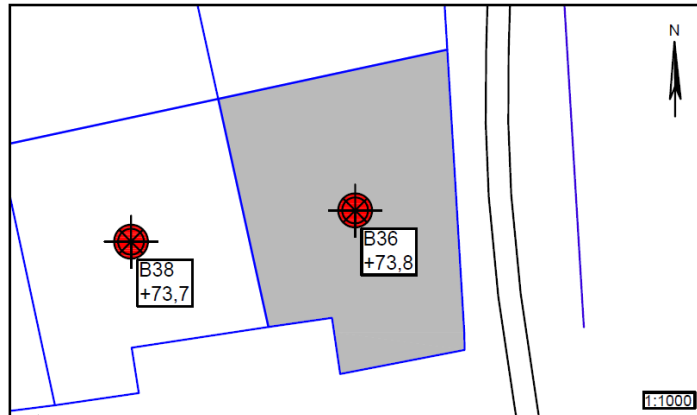
Figur 1 – Situationsplan 1:1000, Hvedebakken 36
