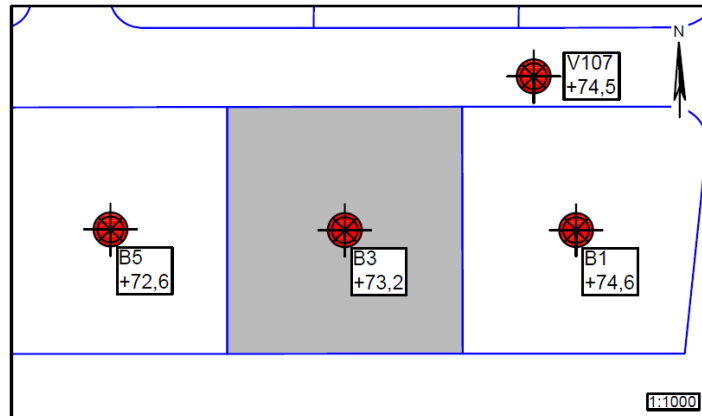
Figur 1 – Situationsplan 1:1000, Hvedebakken 3
