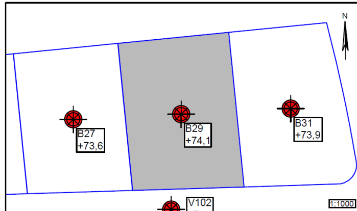
Figur 1 – Situationsplan 1:1000, Hvedebakken 29
