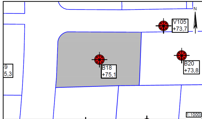
Figur 1 – Situationsplan 1:1000, Hvedebakken 18
