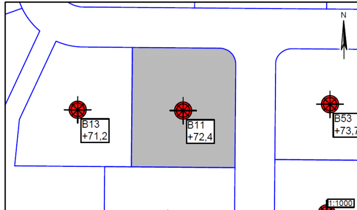
Figur 1 – Situationsplan 1:1000, Hvedebakken 11
